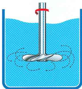
PROPELLER FLOW PATTERN
