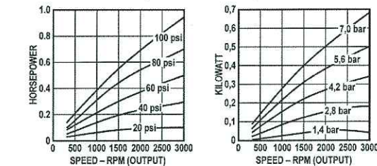
Output Power vs. Speed
